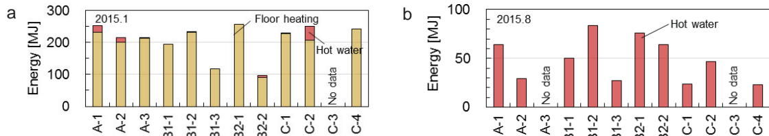
Fig. 12. Collected heat energy by solar system (a) winter (2015.1); (b) summer (2015.8).
