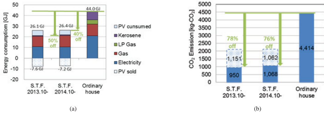
Fig. 8. Energy Performance of ST Fuchu (a) Annual energy consumption; (b) Annual carbon dioxide emissions.
