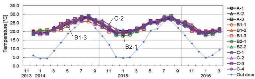
Fig. 5. Monthly average temperature of living room.
