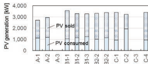
Fig. 11. Electricity generated by PV power system (2014.10-2015.9).
