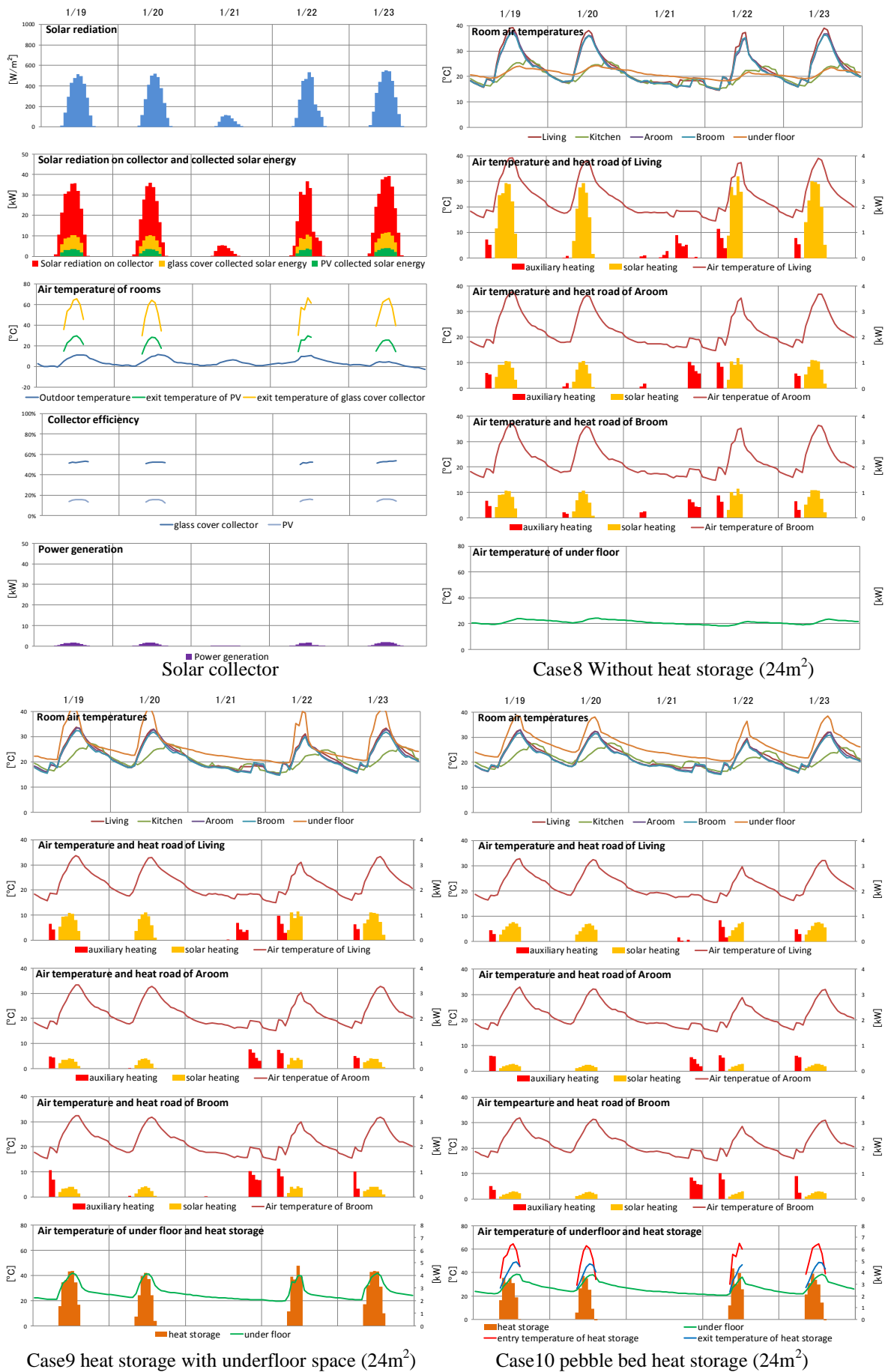
Fig.5. simulation results (Glass collector area 24m 2 1/19-1/23)
